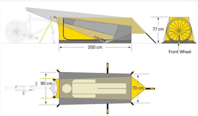
Front Wheel Frame Support
